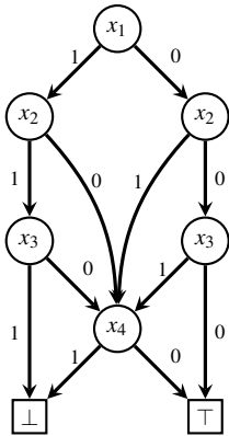
Fig. 2: ROBDD for the PB constraint 2x_1 + 3x_2 + 4x_3 + 6x_4 \leq 7 with variable ordering x_1 \prec x_2 \prec x_3 \prec x_4 .
