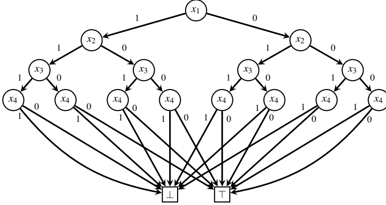
Fig. 1: Non-reduced Ordered BDD for the PB constraint 2x_1 + 3x_2 + 4x_3 + 6x_4 \leq 7 with variable ordering x_1 \prec x_2 \prec x_3 \prec x_4 .
