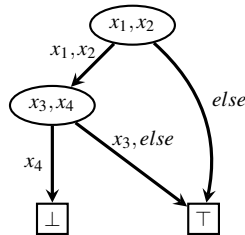
Fig. 3: AMO-ROMDD for 2x_1 + 3x_2 + 4x_3 + 5x_4 \leq 7 , with ordered partition \{x_1, x_2\} \prec \{x_3, x_4\} . Multiple edges between two nodes are represented as a single edge with multiple labels.
